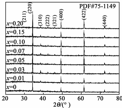
图 1 (\text{Ca}_{0.97}\text{Ba}_{0.03})\text{Cu}_3\text{Ti}_{4-x}\text{Nb}_x\text{O}_{12} 陶瓷的 XRD 图谱
